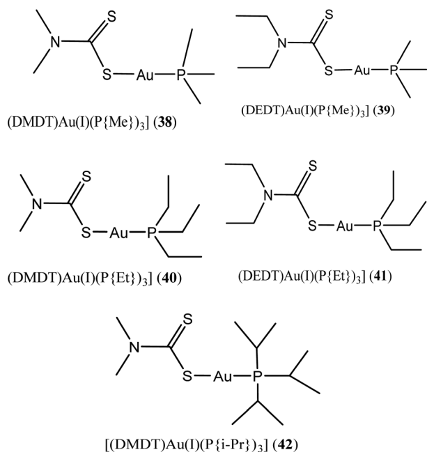
Fig. 9 Chemical structures of novel phosphane-gold(I) dithiocarbamate complexes 38–42.
