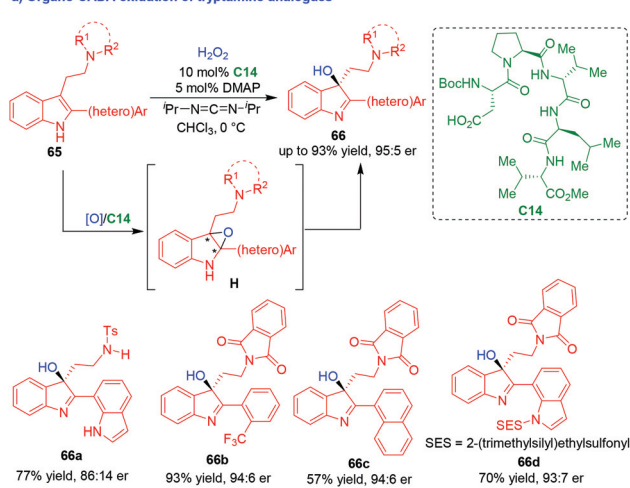
b) Stereoselective rearrangement of C3-hydroxy indolenine into 2-oxindole
