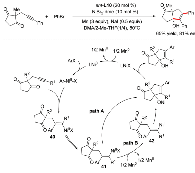
Scheme 31 Ni-Catalyzed enantioselective anti -arylation cyclization of alkynones with aryl halides.
