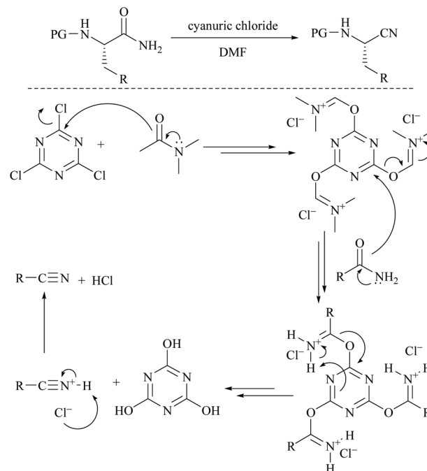
Scheme 11 Cyanuric chloride mediated dehydration.
