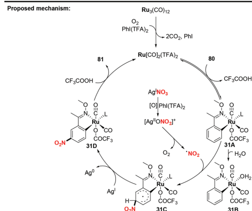
Scheme 31 Ruthenium-catalyzed oxime-directed meta -C Ar -H nitration of arenes.
