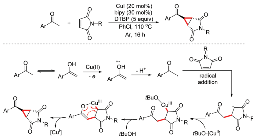
Scheme 49
