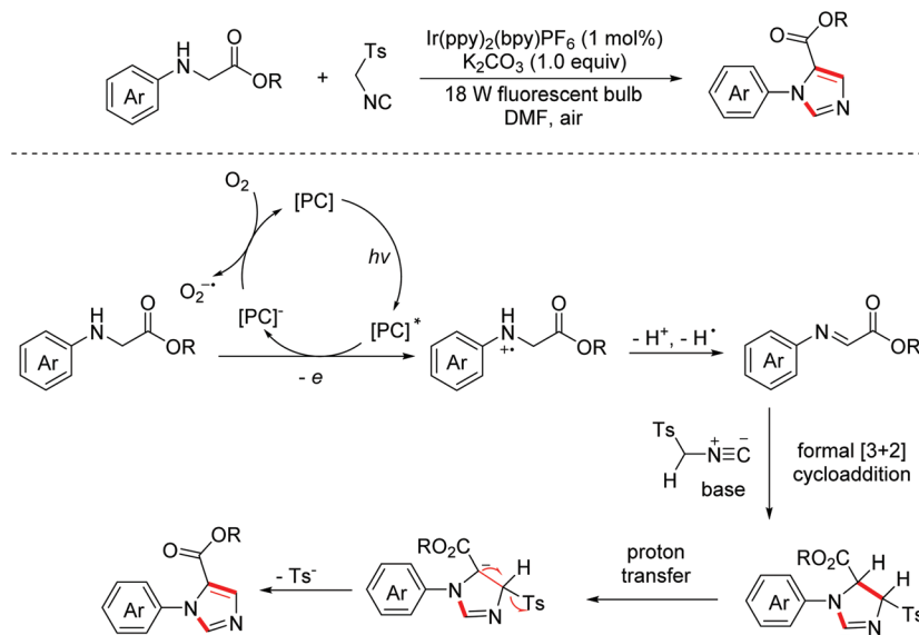
Scheme 4
