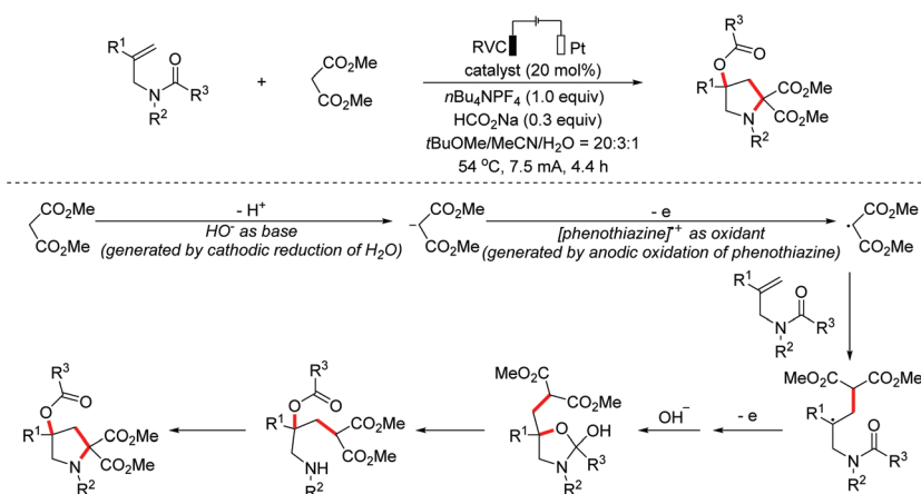
Scheme 20
