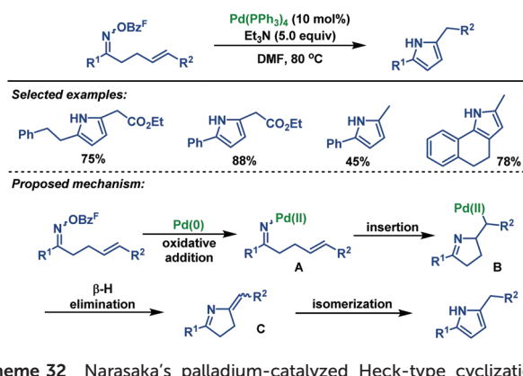
Scheme 32 Narasaka's palladium-catalyzed Heck-type cyclization of \gamma,\delta -unsaturated oxime: synthesis of pyrrole derivatives.
