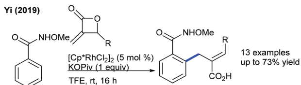
Scheme 138 Allylation of benzamides with methyleneoxetanones.
