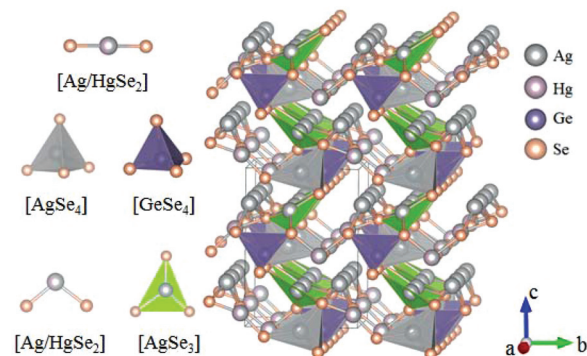
Fig. 27 Crystallographic structure of Ag 6 HgGeSe 6 .
