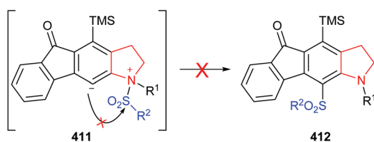
Scheme 57 Mechanistic rationales for desulfonylation of mesyl groups, migration of p -nitrobenzene from nosyl group and inhibition of sulfonyl migration for indoline derivatives.
