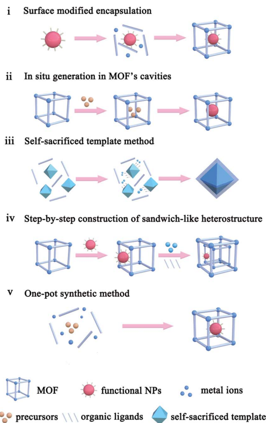
Scheme 1 Main approaches used for the construction of MOF-based composites.
