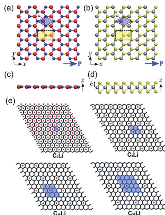
Fig. 3 Top-view geometry of monolayer (a) h-BN and (b) trigonal prismatic molybdenum disulfide (2H-MoS 2 ) (B atoms: blue, N atoms: red, Mo (transition metal) atoms: silver, S (chalcogenide) atoms: yellow). The axes and directions of piezoelectric polarization are designated. The hexagonal primitive cell is marked as blue regions. The orthorhombic unit cell applied in the density functional theory (DFT) simulations is marked as yellow regions. (c and d) Side-view geometry of the atomically thin h-BN monolayer and the 2H-MoS 2 monolayer, respectively. (e) Modelling for different concentrations of Li components doped on graphene layers. Unit cell is marked as blue regions, and expressed by the formula unit C n Li in which n = 2, 8, 18 , and 32 . This figure has been adapted/reproduced from ref. 115 and 125 with permission from American Chemical Society, copyright 2012.
