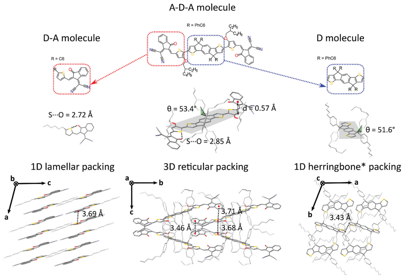
Fig. 2 Chemical structures of IEICO (center) and its subunits: D–A small molecule “ICA” (left) and D molecule “IDT01” (right) small donor molecule. (b) Molecular conformations of ICA, IEICO and IDT01 small molecule in single crystal and representation of the dihedral angle \theta between the side chains and the planar backbone and of the S \cdots O conformational locks. (c) Molecular packing representations for the three structures: 1D \pi – \pi lamellar stacking (ICA), reticular arrangement with a 3D \pi – \pi connectivity (IEICO) and herringbone motif with no \pi – \pi overlap (IDT01).
