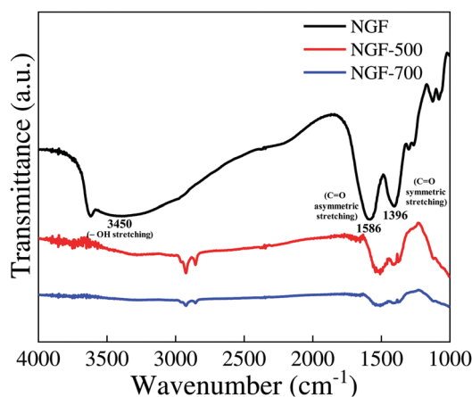
Fig. 5 FTIR spectra of the as-prepared (NGF), 500 °C (NGF-500) and 700 °C (NGF-700) annealed NaGdF 4 :3% Tb 3+ phosphor crystals.
