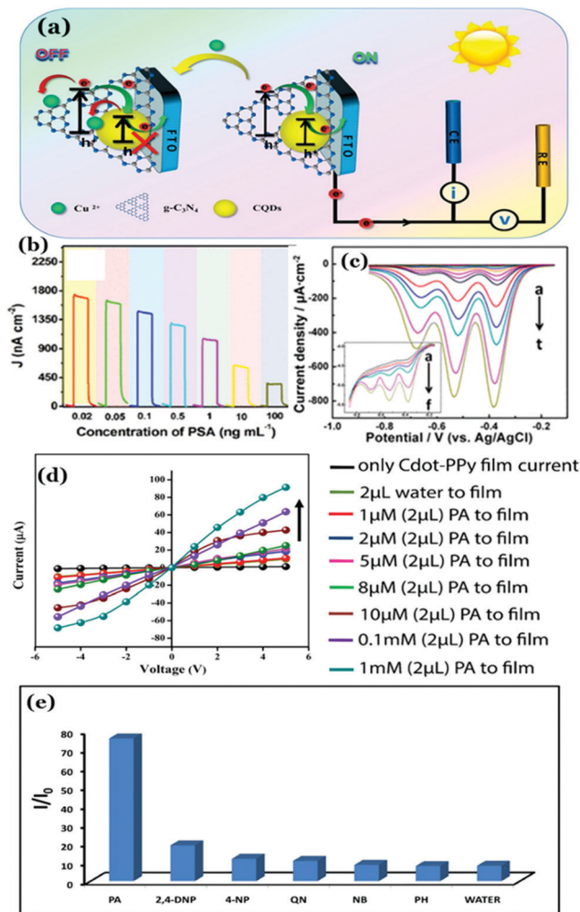
Fig. 15 (a) Mechanism of Cu^{2+} -quenched photocurrent of Cdote/g- C_3N_4 heterostructures. (b) Photocurrent responses of the Cdote/g- C_3N_4 sensing platform towards prostate-specific antigen (PSA) with different concentrations. Reprinted with permission from ref. 240. Copyright 2017 American Chemical Society. (c) Differential pulse voltammograms (DPVs) responding to different concentrations of TNT at the CDs/GC electrode. Reprinted with permission from ref. 244. Copyright 2015 American Chemical Society. (d) I - V characteristics of the Cdote-PPy composite film in the presence of different concentrations of picric acid (PA) solutions. (e) The ratios of current flowing through the composite film following addition of 2.0 \mu L 1.0 mM aqueous solution of different analytes. In the figure PA = picric acid, 2,4-DNP = 2,4-dinitrophenol, 4-NP = 4-nitrophenol, NB = nitrobenzene, PH = phenol, QN = 1,4-benzoquinone, 4-MBA = 4-methoxybenzoic acid. The measurements were made at +5 V. Reprinted with permission from ref. 119. Copyright 2016 American Chemical Society.
