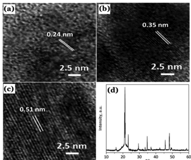
Fig. 10 (a–c) Observed lattice planes in the as-prepared Cdots reported by Sun et al. (d) Powder XRD pattern of the Cdots. Reproduced with permission ref. 126. Copyright 2015 Royal Society of Chemistry.
