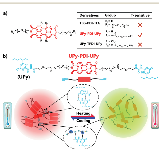
Scheme 1 (a) Molecular structure of three PDI derivatives; 2. (b) Schematic illustration of temperature-sensitive supramolecular fluorescent nano-assemblies.
