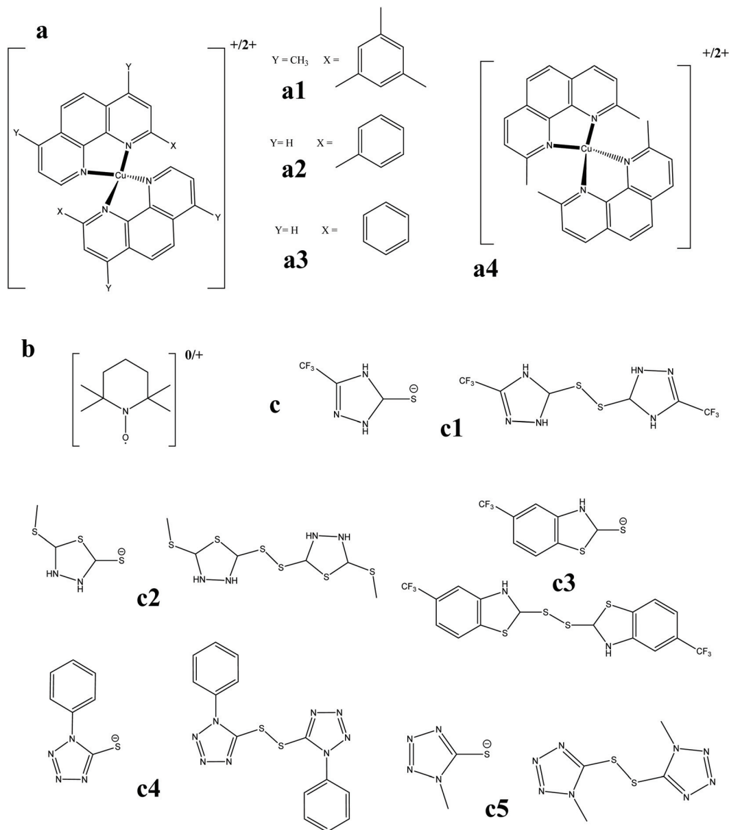
Fig. 6 Chemical structures of various alternative redox couples: (a) copper-based complexes (a1: [\text{Cu}(\text{2-mesityl-4,7-dimethyl-1,10-phenanthroline})]^{+/2+} ; a2: [\text{Cu}(\text{2-tolyl-4,7-dimethyl-1,10-phenanthroline})]^{+/2+} ; a3: [\text{Cu}(\text{2-phenyl-4,7-dimethyl-1,10-phenanthroline})]^{+/2+} ; and a4: [\text{Cu}(\text{2,9-dimethyl-1,10-phenanthroline})]^{+/2+} ), (b) TEMPO ^{0/+} (2,2,6,6-tetramethyl-1-piperidinyloxy) and (c) sulphur-based organic molecules: (c1: 2-methyl-5-trifluoromethyl-2H-[1,2,4]triazole-3-thiol and 3,3'-dithiobis(2-methyl-5-trifluoromethyl-2H-[1,2,4]triazole); c2: 5-(methylthio)-1,3,4-thiadiazolidine-2-thiolate and 1,2-bis(5-(methylthio)-1,3,4-thiadiazolidin-2-yl)disulfane; c3: 5-(trifluoromethyl)-2,3-dihydrobenzo[d]thiazole-2-thiolate and 1,2-bis(5-(trifluoromethyl)-2,3-dihydrobenzo[d]thiazol-2-yl)disulfane; c4: 1-phenyl-1H-tetrazole-5-thiolate and 1,2-bis(1-phenyl-1H-tetrazol-5-yl)disulfane; and c5: 5-mercapto-1-methyl tetrazole and di-5-(1-methyltetrazoledisulfide)). All molecules were drawn using ChemDraw 19.0.
