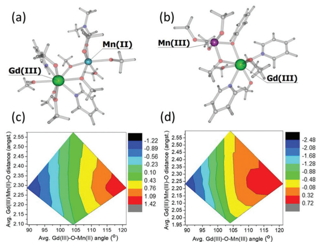
Fig. 7 Models 3_{\text{Mn(II)-Gd(III)}} (a) and 3_{\text{Mn(III)-Gd(III)}} (b) together with the magneto-structural correlation contour plots (c) and (d) performed by varying the average Mn(II)/Mn(III)-O-Gd(III) angle and average Mn(III)/Gd(III)-O distance with respect to the magnetic exchange coupling constants J_{\text{Mn(II)-Gd(III)}}^{\text{exchange}} and J_{\text{Mn(III)-Gd(III)}}^{\text{exchange}} . The keys represent the magnitude of the exchange, ranging from most antiferromagnetic (black) to most ferromagnetic (red). For both models, the change in the magnitude of the interaction with respect to the change in Mn(III)-O-Gd(III)-O dihedral angle is minimal. See Fig. S3 of the ESI for more details.†
