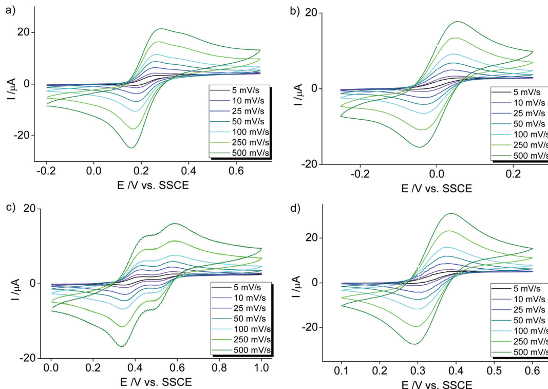
Fig. 5 Cyclic voltammograms of homoleptic [\text{Co}(\text{pyPYA}_2)_2](\text{PF}_6)_2 complexes in MeCN: (a) 2a [\text{Co}(\text{para-pyPYA}_2)_2](\text{PF}_6)_2 ; (b) 2b [\text{Co}(\text{meta-pyPYA}_2)_2](\text{PF}_6)_2 ; (c) 2c [\text{Co}(\text{ortho-pyPYA}_2)_2](\text{PF}_6)_2 ; (d) [\text{Co}(\text{terpy})_2](\text{PF}_6)_2 . Conditions: 10 mL solvent, 1 mM sample and 100 mM (n\text{Bu}_4\text{N})\text{PF}_6 as supporting electrolyte at 5–500 \text{mV s}^{-1} scan rate (potentials vs. Ag/AgCl using the \text{Fc}^+/\text{Fc} couple as standard; E_{1/2} = +0.4319 ).
