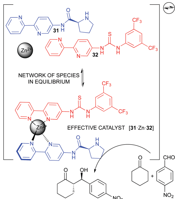
Fig. 17 Dynamic network of organocatalytic bipyridine ligands templated by \text{Zn(II)} .
