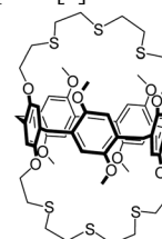
Pillar[5]-bis-trithiacrown (L)
