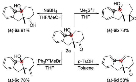
Scheme 2 Derivatization of bicyclic product 2a .
