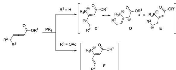
Scheme 1 The reactivity of allenooates in the presence of organophosphines.
