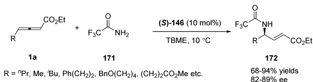
Scheme 53 Phosphine-catalysed \gamma -addition of trifluoromethyl-amide to \gamma -substituted allenoates.
