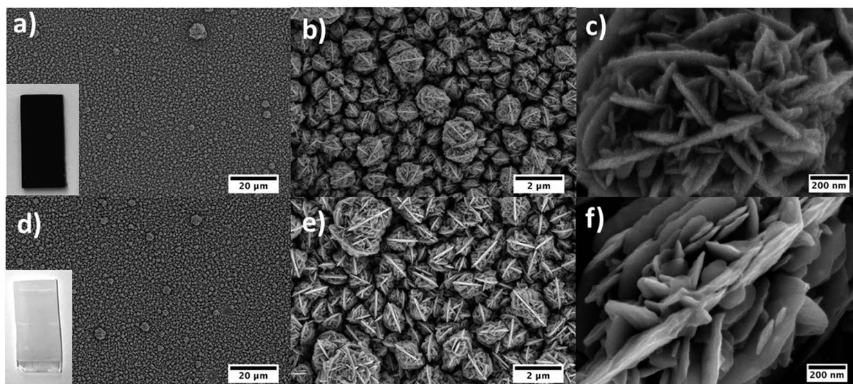
Fig. 2 SEM micrographs of \text{TiO}_2 photoanodes grown by AACVD. (a–c) \text{TiO}_2 -Rose-AD and (d–f) \text{TiO}_2 -Rose-800. Insets in (a) and (d) show photographs of \text{TiO}_2 -Rose-AD and \text{TiO}_2 -Rose-800 photoanodes, respectively.
