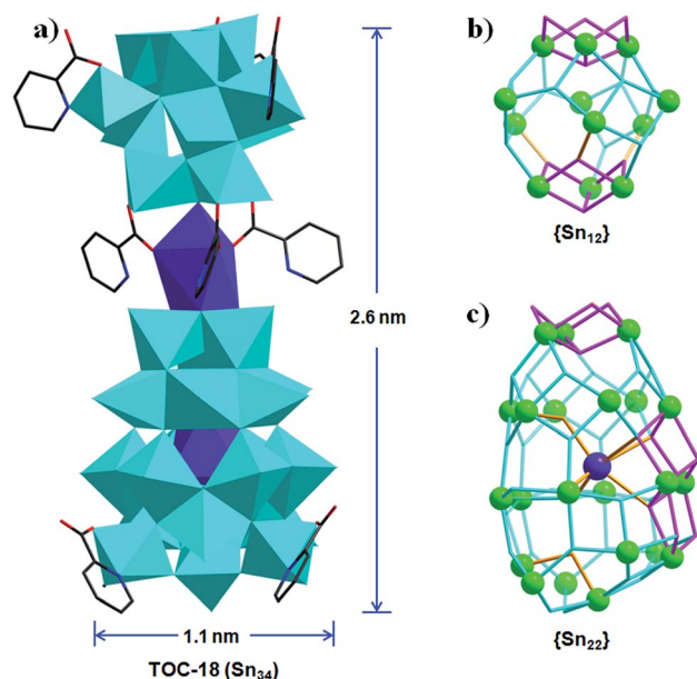
Fig. 3 (a) The polyhedral representation of TOC-18 . (b) and (c) The ball-and-stick representations of \{\text{Sn}_{12}\} and \{\text{Sn}_{22}\} moieties in TOC-18 . Polyhedral color code: blue \text{SnO}_5\text{C}/\text{SnO}_4\text{C}/\text{SnO}_4\text{NC} ; purple \text{NaO}_7/\text{NaO}_6 . Atom color code: green Sn; purple Na; red O; black C; dark blue N.
