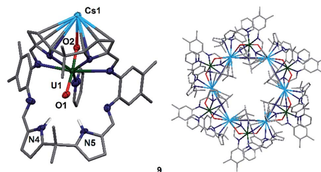
Fig. 6 Solid state structure of 9 , depicting the asymmetric unit (left) and the hexanuclear Cs + –uranyl(v) ring (right). For clarity, all hydrogen atoms except pyrrole N–Hs and all solvent molecules are omitted (displacement ellipsoids are drawn at 50% probability). Selected bond distances (Å) and angles (°): U1–O1 1.857(6), U1–O2 1.833(6), O1–N4 3.01(1), O1–N5 2.92(1), O1–U1–O2: 175.2(3)°, Cs1–O2–U1 117.6(3)°; selected ring parameters (Å): Cs1–Cs1''' 13.4807(9), U1–U1''' 16.518(1); cavity size: 648 Å 3 .
