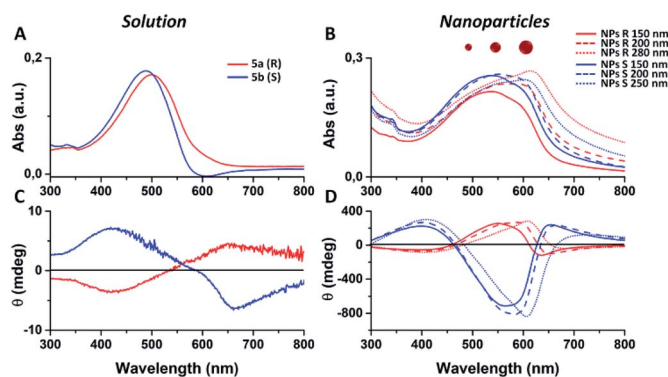
Fig. 2 (A and C) Absorption and circular dichroism spectra of polymers 5a (R, red line) and 5b (S, blue line) in \text{CHCl}_3 . (B and D) Absorption and circular dichroism spectra of NPs obtained from polymers 5a (R, red lines) and from polymer 5b (S, blue lines).
