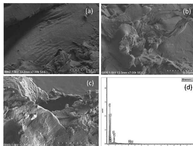
Fig. 10 FESEM images of (a) fresh wood chips (5 \mu\text{m} ), (b) used wood chips (5 \mu\text{m} ), and (c) used wood chips (10 \mu\text{m} ). (d) Elemental mapping from EDX of used date seed (25 \mu\text{m} ).
