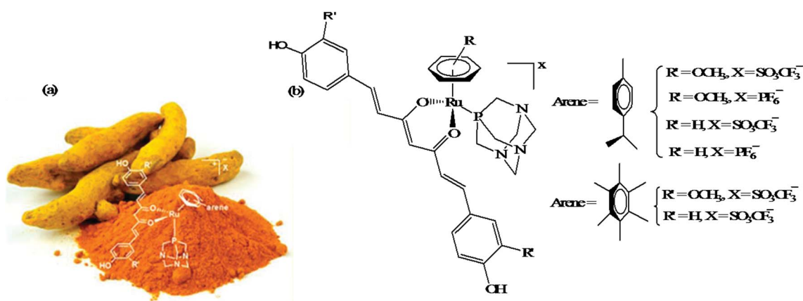
Fig. 11 (a) Curcuma longa- (turmeric) and (b) ruthenium(II) arene RAPTA-type complexes [Ru( \eta^6 - p -cymene)(curc)-(PTA)]X and [Ru(hmb)-(curc)(PTA)]X derived from curcumin. (a) was reproduced from its original paper after taking the copyright from ACS. This figure was taken from ref. 72, which is an open access article published under an ACS Author Choice License, which permits copying and redistribution of the article or any adaptations for non-commercial purposes.
