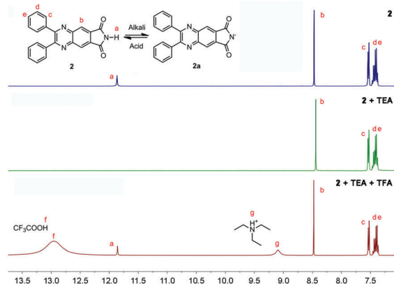
Fig. 10 ^1\text{H-NMR} spectra of 2 before and after the addition of excess TEA and TFA.
