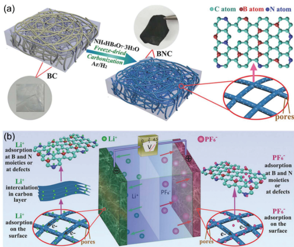
Fig. 9 Example of an advanced non-aqueous hybrid capacitor: A LIC using B and N dual-doped carbon nanofibers as both the cathode and the anode. (a) Schematic of the fabrication process of BNC. (b) Schematic of the charge-storage mechanisms of BNC//BNC LIC. Reproduced with permission from ref. 100. Copyright 2017, Wiley-VCH.
