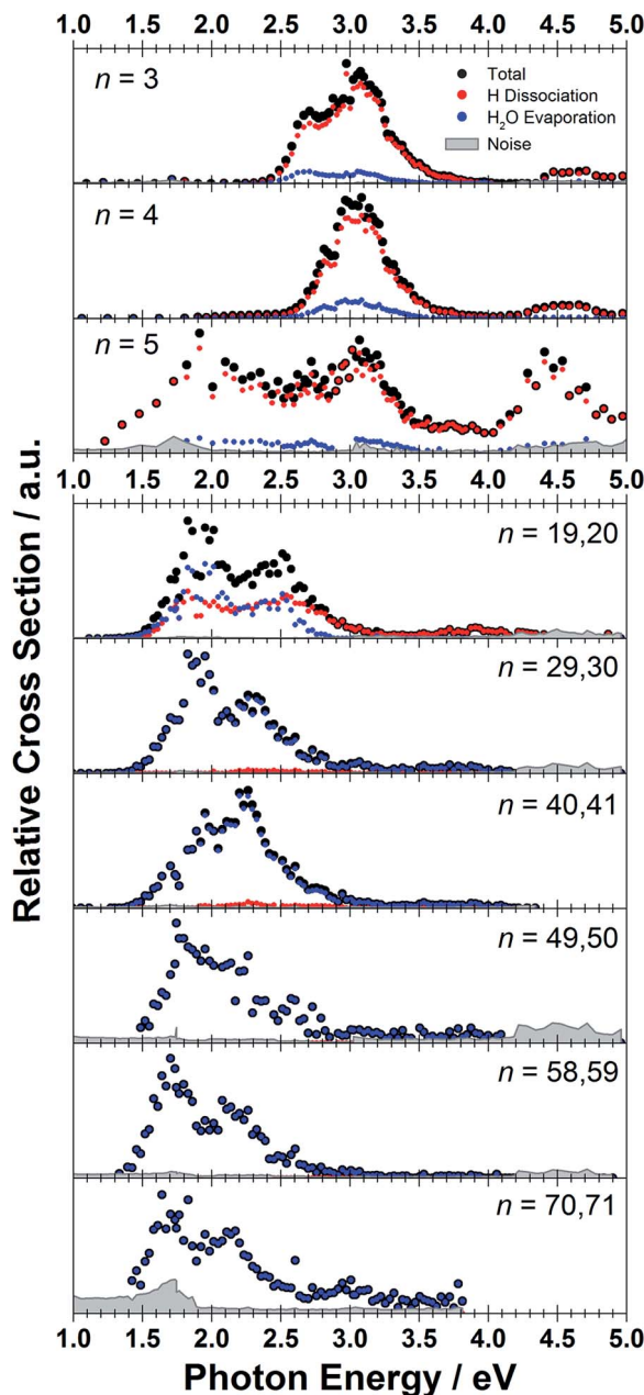
Fig. 1 Experimentally measured relative photodissociation cross sections of [\text{Mg}(\text{H}_2\text{O})_n]^+ ions for 3 \leq n \leq 5 (adapted from ref. 42) and n \sim 20, 30, 40, 50, 60 and 70 , with partial cross sections for fragmentation via only the loss of water molecules (blue) and the additional loss of atomic hydrogen (red).
