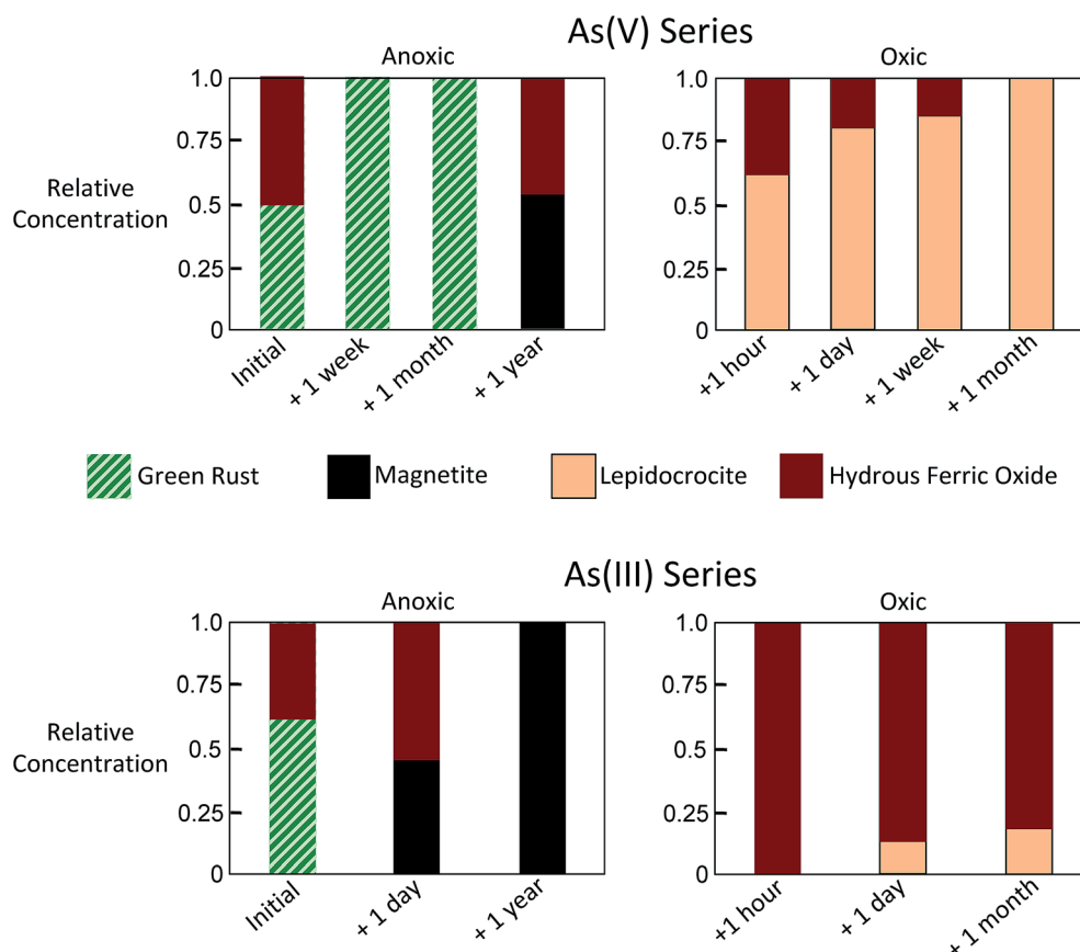
Fig. 4 Relative concentrations of Component 1 (green rust), Component 2 (magnetite), Component 3 (lepidocrocite) and Component 4 (hydrous ferric oxide) derived by ITFA.
