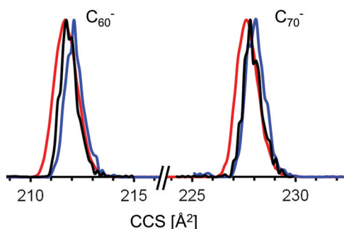
Fig. 3 Typical mobilograms of C 60 − and C 70 − recorded in the same measurement runs on three different days. Identical colors indicate identical runs. Within the same run, peak maxima can be determined to a relative accuracy of significantly better than 0.5%. 38
