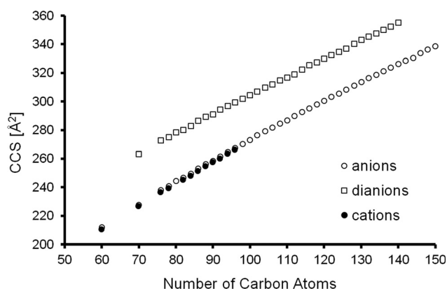
Fig. 2 Experimental ^{TIMS}CCS_{N_2} of fullerene ions in the size range between 60 and 150 atoms (in three different charge states as indicated). The standard deviation is ca. 0.5% or 1 Å 2 which corresponds to the size of the symbols.
