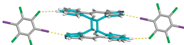
Fig. 4 X-ray structure of the partially photoreacted co-crystal of form I forming the ht -PP shown in turquoise. The I...N halogen bonds and C-H...Cl contacts are shown with yellow dashed lines.
