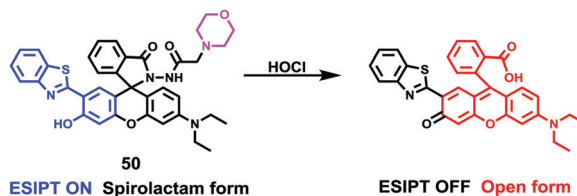
Scheme 37 Fluorescent probe 50 for HOCl.
