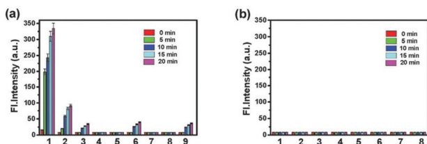
Fig. 108 (a) Time-dependent fluorescence response of 2\ \mu\text{M} 65 to the testing species in HEPES buffer solution (10 mM, 0.5% DMSO, 0.5% TW 80, pH 5.0): 1, 10\ \mu\text{M} AS; 2, 20\ \mu\text{M} GSNO; 3, 200\ \mu\text{M} ONOO - ; 4, 50\ \mu\text{M} NOC-5; 5, 500\ \mu\text{M} NO 2 - ; 6, 200\ \mu\text{M} H 2 O 2 ; 7, 100\ \mu\text{M} O 2 - ; 8, 20\ \mu\text{M} MeLOOH; 9, 200\ \mu\text{M} ClO - . (b) 1, 50\ \mu\text{M} L-cys; 2, 100\ \mu\text{M} GSH; 3, 500\ \mu\text{M} NaHS; 4, 200\ \mu\text{M} ascorbic acid; 5, 200\ \mu\text{M} tocopherols; 6, 100\ \mu\text{M} citrate; 7, 200\ \mu\text{M} tyrosine (Tyr); 8, 50\ \mu\text{M} hydroxylamine (HA). Bars represent fluorescence intensity during 0, 5, 10, 15, and 20 min after addition of various compounds. \lambda_{\text{ex}} = 690\ \text{nm} , \lambda_{\text{em}} = 700\ \text{nm} . Copyright 2014 Royal Society of Chemistry.
