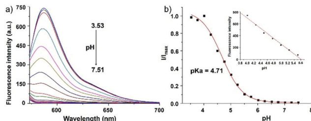
Fig. 5 (a) Fluorescence spectra of probe 3 (10 \mu\text{M} ) in buffer at various pH values; (b) fluorescence intensity at 584 nm with pH values according to the fluorescent pH titration (pH 3.53–7.51), \lambda_{\text{ex}} = 563 nm. The inset shows the linear relationship of fluorescence intensity at 584 nm and pH values from 4.0 to 5.5 ( R = 0.98101 ). Copyright 2013 Elsevier.
