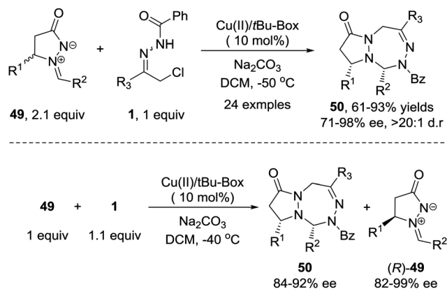
Scheme 22 Cu(II)-Catalyzed asymmetric 1,3-dipolar [4+3] cycloaddition and kinetic resolution of azoalkenes with azomethine imines.
