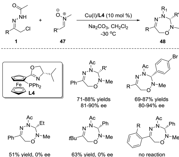
Scheme 21 Cu(I)-Catalyzed asymmetric 1,3-dipolar [4+3] cycloaddition of azoalkenes with nitrones and its limitations.
