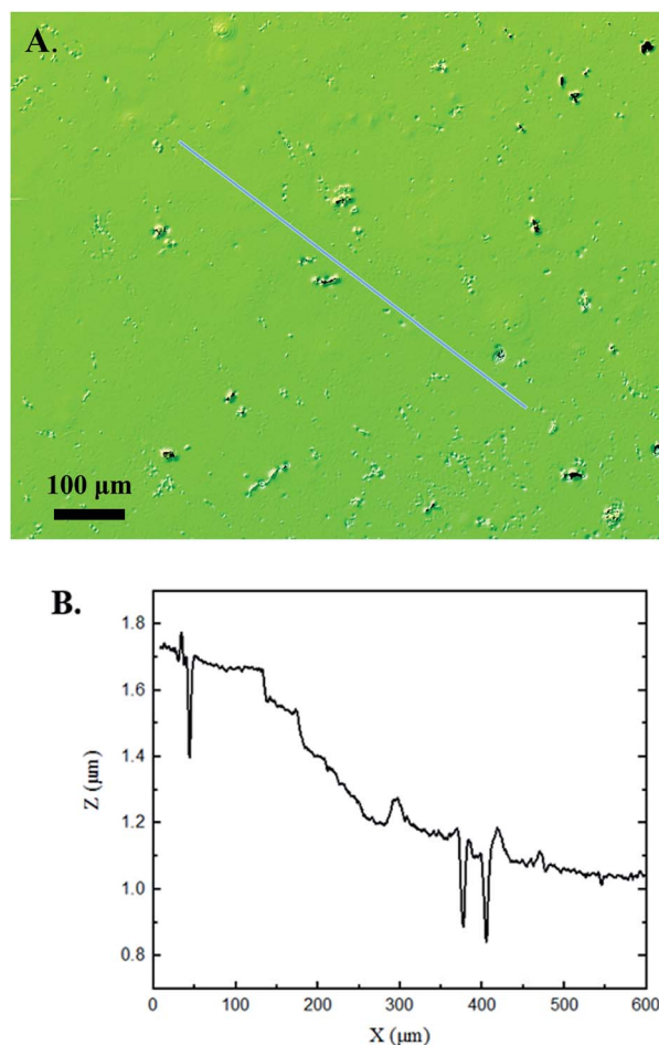
Fig. 6 Interferometry analysis of an experimental PDMS sample. (A) The surface has a roughness texture that is visually different from that in the control images. (B) The graphical height displacement across an arbitrary line on the surface shows abrupt spikes in the z direction below the surface, pointing to signs of cavitation damage.
