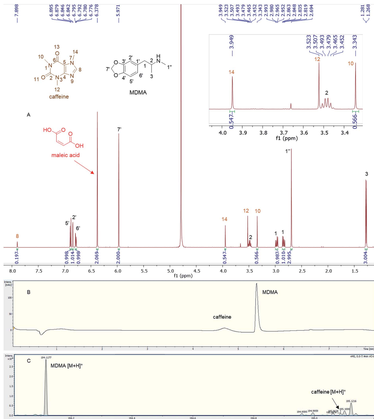
Fig. 4 (A) 1 H NMR (in D 2 O) of tablet 11a showing the caffeine peaks with expansion of the region between 3.4–4.5 ppm, (B) UHPLC of tablet 11a showing a broad peak for caffeine at RT = 4.7 min, (C) MS trace of tablet 11a showing MDMA molecular ion and caffeine low intensity molecular ion at 195.0874 m/z.
