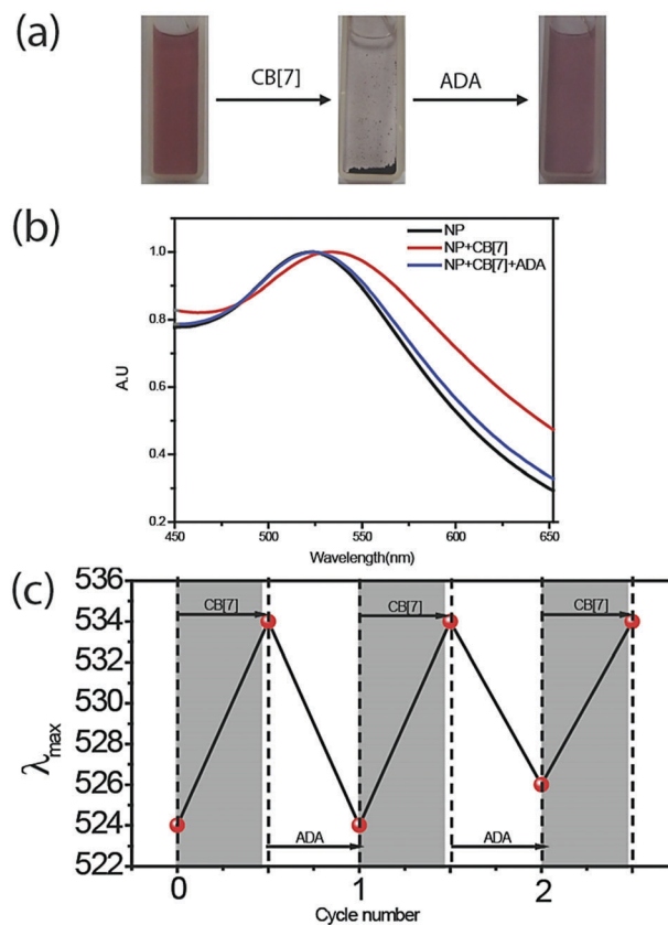
Fig. 1 (a) Reversible assembly of AuNPs. Assembly driven by supramolecular interaction between AuNP and CB[7], and disassembly driven by high affinity guest ADA. 200 nM AuNPs were used to form the assemblies. (b) UV-Vis spectroscopy study of the NP assembly and disassembly process. NP plasmon absorption maximum shifted to the right side in the case of NP + CB[7] and the absorption maximum again came back to the initial stage in the case of NP + CB[7] + ADA. A relatively lower concentration (37 nM) of AuNP was used for this study to achieve smaller and dispersed assembly. (c) Reversible changes in absorption maximum of 5 nm AuNPs by alternative addition of CB[7] and ADA.
