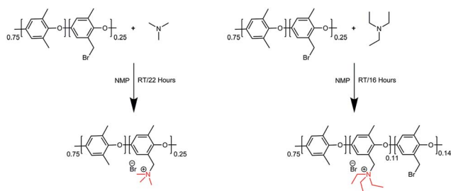
Scheme 2 Preparation of PPO-TMA and PPO-TEA polymers.
