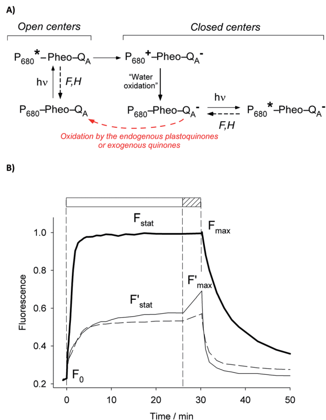
Fig. 3 (A) Overview of the different pathways within Photosystem II after light excitation. Relaxation can occur by fluorescence ( F ) or heat ( H ) emission (such pathways mainly include relaxations of excited chlorophyll antenna; see the Fig. 1 legend. For more clarity, only the decays from the excited state of P_{680} are displayed). Additionally, a charge separation occurs from the reduction of the primary acceptor Q_A by P_{680} through pheophytin (Pheo). The oxidized P_{680}^+ then induces the oxidation of water. The electron transfer along the chain will then proceed by means of the plastoquinone pool (see Fig. 1). Exogenous quinones are PSII acceptors and can extract photosynthetic electrons by oxidizing Q_A^- or the plastoquinone pool. (B) Fluorescence induction curves (see the text) achieved with a suspension of Chlamydomonas reinhardtii ( \Delta petA mutants; 10^7 cells per mL). The solid lines correspond to typical curves without any addition of exogenous quinones (solid thick line) or in the presence of 2,6 DCBQ (solid thin and dashed lines; 25 \mu\text{mol L}^{-1} ). The thin solid line corresponds to a curve recorded just after the addition of quinones. The dashed line displays the induction curve after 3 h of pre-incubation with the quinone. The fluorescence values are normalized with respect to the maximum value F_{max} . The shape of the induction curve is related to the illumination sequence. Firstly, a continuous illumination is applied (top rectangle in white). The initial fluorescence level, F_0 , is related to a situation in which all the Q_A centers are in an oxidized state ((A) left). Then, the photosynthetic activity begins. Some open Q_A centers are reduced to closed Q_A^- centers which may be oxidized by endogenous plastoquinones or exogenous quinones ((A) right). This leads to a higher steady-state fluorescence level ( F_{stat} ) that results from the relaxation of open ( Q_A ) and closed ( Q_A^- ) centers ((A) left and right). Secondly, the saturating pulse (top hatched rectangle) prevents the oxidation of Q_A^- , thus leading to a maximum fluorescence level ( F_{max} ).
