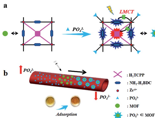
Scheme 1 Schematic diagram for the treatment of hyperphosphatemia based on Zr(IV) -MOFs. (a) Proposed mechanism of the fluorescence nanosensor for phosphate; (b) reduced levels of phosphate by MOFs for highly efficient treatment of hyperphosphatemia.
