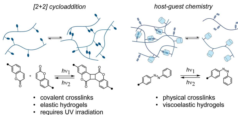
Fig. 1 (a) Previous strategies for photoreversible control over hydrogel mechanics rely on photocycloadditions or supramolecular complexes with photoswitch guests. (b) In this work, the configuration of an adjacent photoswitch controls the stability of a dynamic covalent crosslink, thus reversibly tuning mechanics with light.
