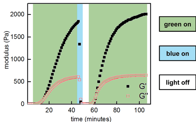
Fig. 6 Photocontrolled cycling of hydrogel viscoelasticity (10% strain, 25 \text{ rad s}^{-1} ) of P1 and P2-F 2 (1 : 1, 10 w/v% in PBS, pH 7.5). Green light induces gelation, and blue light induces softening.
