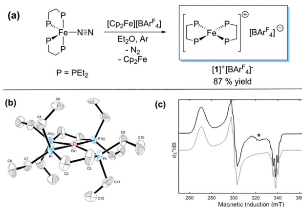
Fig. 1 (a) Synthesis of [1]^+[\text{BAR}_4^{\text{F}}]^- . (b) ORTEP diagram of the [\text{Fe}(\text{depe})_2]^+ fragment in [1]^+[\text{BAR}_4^{\text{F}}]^- ; thermal ellipsoids shown at 30% probability, H atoms and [\text{BAR}_4^{\text{F}}]^- counterion omitted for clarity (C and P occupancies are 0.5 as a consequence of a second symmetry-generated orientation of the two depe ligands; this has also been omitted for clarity). (c) CW X-band ESR spectrum of [1]^+[\text{BAR}_4^{\text{F}}]^- ( \text{PhMe} : \text{DFB} 7 : 1 ; \text{Ar} ; 40 K); black line: experiment; grey line: simulation. * [1 \cdot \text{N}_2]^+[\text{BAR}_4^{\text{F}}]^- impurity due to trace \text{N}_2 in the \text{Ar} atmosphere.
