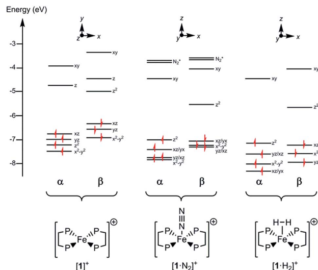
Fig. 9 Electronic energy levels and their occupancy for [\mathbf{1}]^+ , [\mathbf{1}\cdot\mathbf{N}_2]^+ and [\mathbf{1}\cdot\mathbf{H}_2]^+ . The principal Fe character is indicated.
