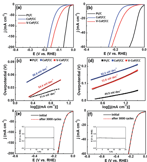
Fig. 5 (a) and (b) HER polarization curves of bare Pt/C, CoP/CC, and V-CoP/CC in 0.5 M \text{H}_2\text{SO}_4 and 1 M PBS, respectively. (c and d) The corresponding Tafel of the catalysts in 0.5 M \text{H}_2\text{SO}_4 and 1 M PBS, respectively. (e and f) Polarization curves of V-CoP/CC at the first cycle and after 3000 cycles in 0.5 M \text{H}_2\text{SO}_4 and 1 M PBS, respectively, and the insets is the chronopotentiometric curve with a constant current density of 10 \text{ mA cm}^{-2} for 25 h in 0.5 M \text{H}_2\text{SO}_4 and 1 M PBS, respectively.
