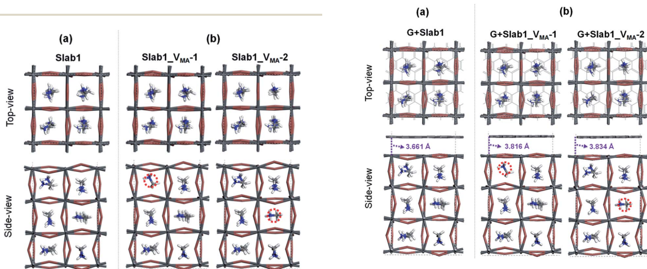
Fig. 17 (a) Defect-free and (b) V_{MA} -containing defective graphene + MAPbI_3 hybrids.
