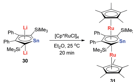
Scheme 18 Synthesis of μ-η⁵:η⁵-stannole dianion complexes 31.
