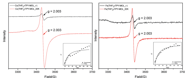
Fig. 6 X-band EPR spectra of \text{Co}(\text{THF})_2 \cdot \text{TPY-MOL} (left) and \text{Fe}(\text{THF})_2 \cdot \text{TPY-MOL} (right) suspended in toluene at r.t. and 20 K. Microwave frequency: 9.629 GHz for \text{Co}(\text{THF})_2 \cdot \text{TPY-MOL} at r.t.; 9.629 GHz for \text{Co}(\text{THF})_2 \cdot \text{TPY-MOL} at 20 K; 9.634 GHz for \text{Fe}(\text{THF})_2 \cdot \text{TPY-MOL} at r.t.; 9.630 GHz for \text{Fe}(\text{THF})_2 \cdot \text{TPY-MOL} at 20 K. Insets are temperature-dependent EPR intensity plots and their fits to the Bleaney and Bowers equation. The fitting results gave a singlet to triplet ( \text{TPY}^{\bullet\bullet} ) ^{2-} energy gap of 0.04 and 0.10 \text{kcal mol}^{-1} for \text{Co}(\text{THF})_2 \cdot \text{TPY-MOL} (left) and \text{Fe}(\text{THF})_2 \cdot \text{TPY-MOL} , respectively.
