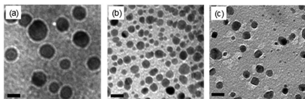
Fig. 2 TEM images of PBNPs prepared from FeCl 2 and K 3 Fe(CN) 6 (a), FeCl 3 , K 3 Fe(CN) 6 , glucose, and GOx (b), FeCl 3 , K 3 Fe(CN) 6 and H 2 O 2 (c). Reaction conditions: 0.25 mM FeCl 3 , 0.25 mM K 3 Fe(CN) 6 , 0.05 mg mL -1 GOx, 1 mM glucose and 1 mM H 2 O 2 in 50 mM MES (pH 3.0) at 25 °C. Scale bar: 20 nm.
